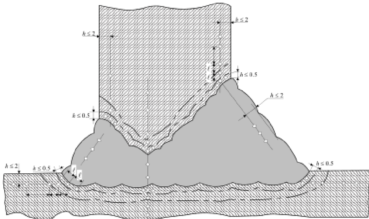
FIGURE 4B Example Showing the Position of the Indentations for Hardness Test on the Weld Metal, the Heat Affected Zone and the Base Metal of a T-Joint Weld (dimensions in mm)
