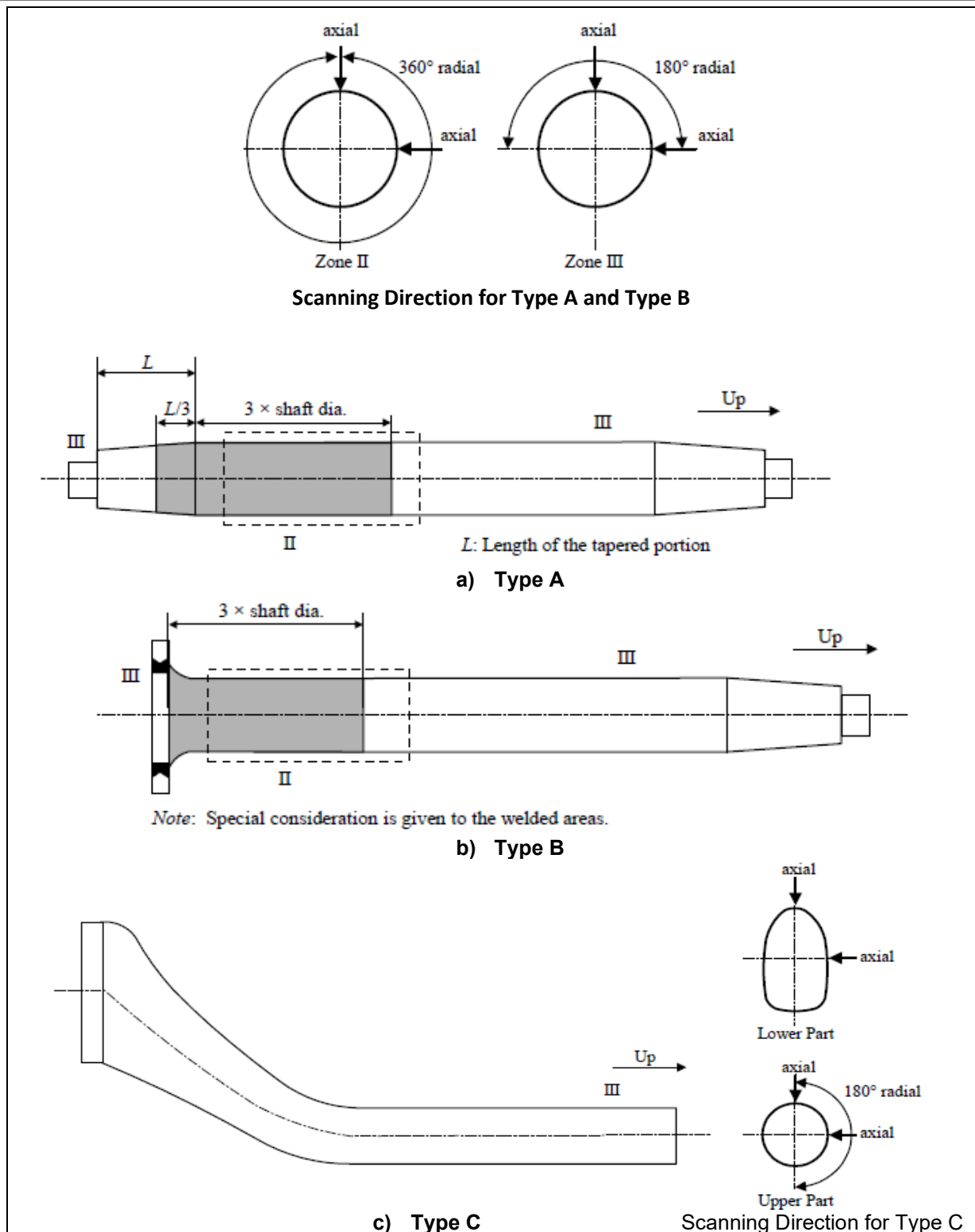
Figure 7.6.8: Zones for Ultrasonic Testing on Rudder Stocks
