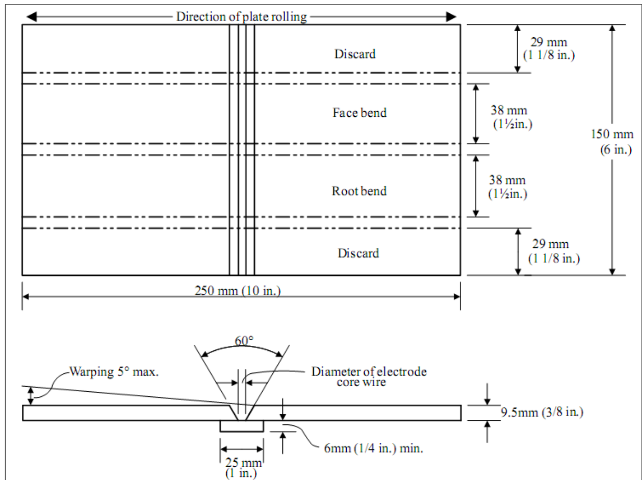
Figure 3.5.9 - Welder Qualification Test No. Q1 For Plate Material 19.0 mm (3/4 in.) or less
