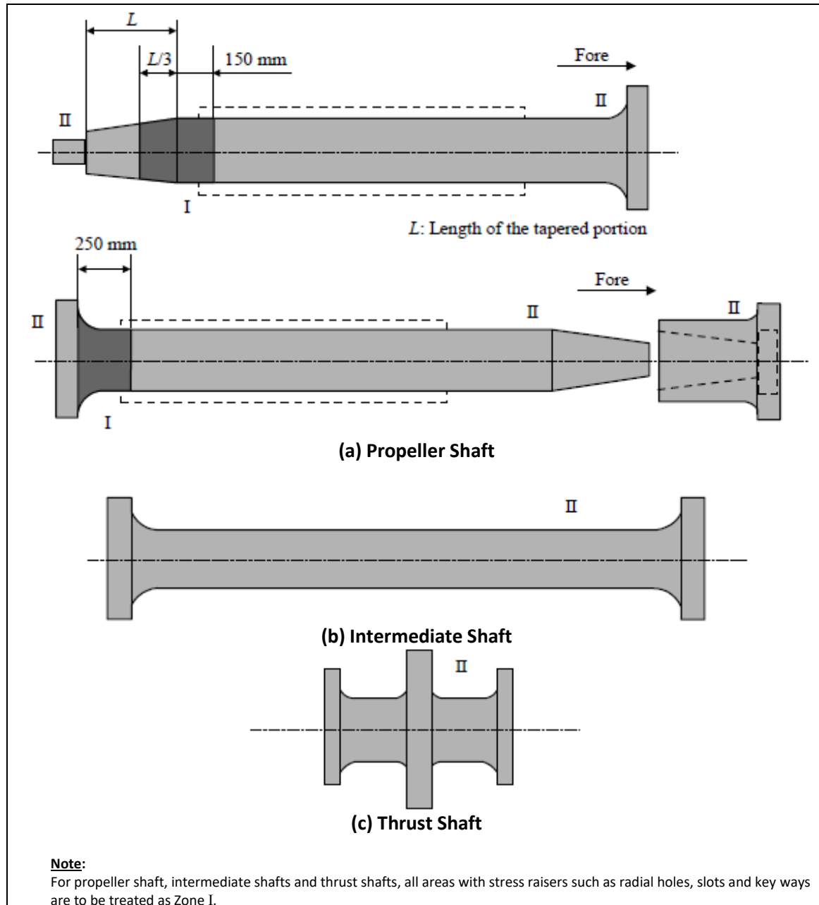
Figure 7.6.2: Zones for Magnetic Particle/Liquid Penetrant Testing on Shafts
