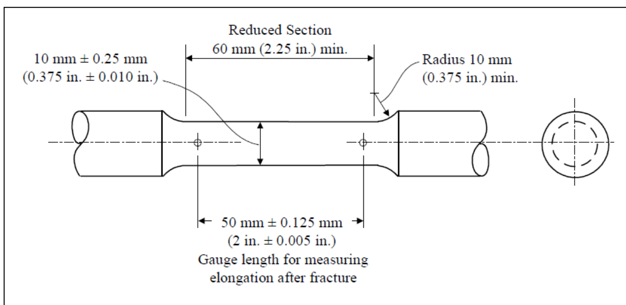
Figure 1.1.3: Standard Round Tension Test Specimen with 50 mm (2 in.) Gauge Length
