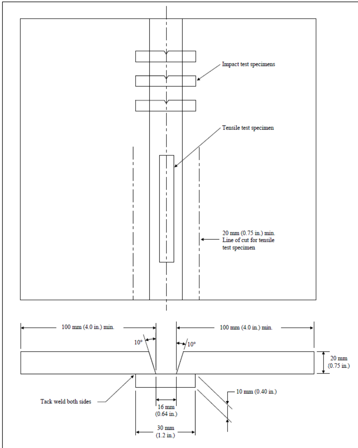
Figure 3.6.5: Deposited-Metal Test Assembly for Manual and Gas-Metal Arc Welding
