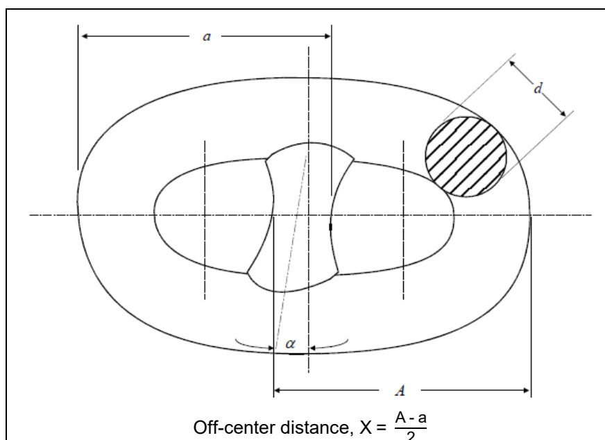
Figure 2.12.2: Final link
