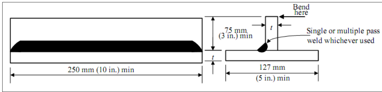
Figure 3.5.8: Test No. 3 – Fillet-weld Test
