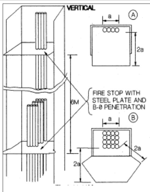
Figure 6.4.2: Non totally enclosed trunks – vertical
