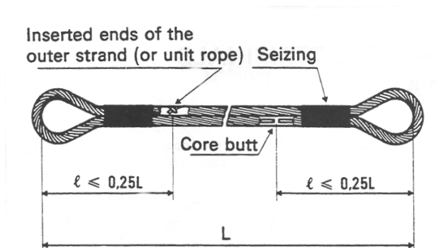
Figure 2.3.15: Double sling
