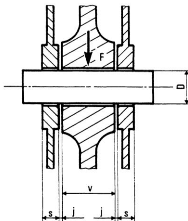
Figure 3.4.4: Axle Pin
