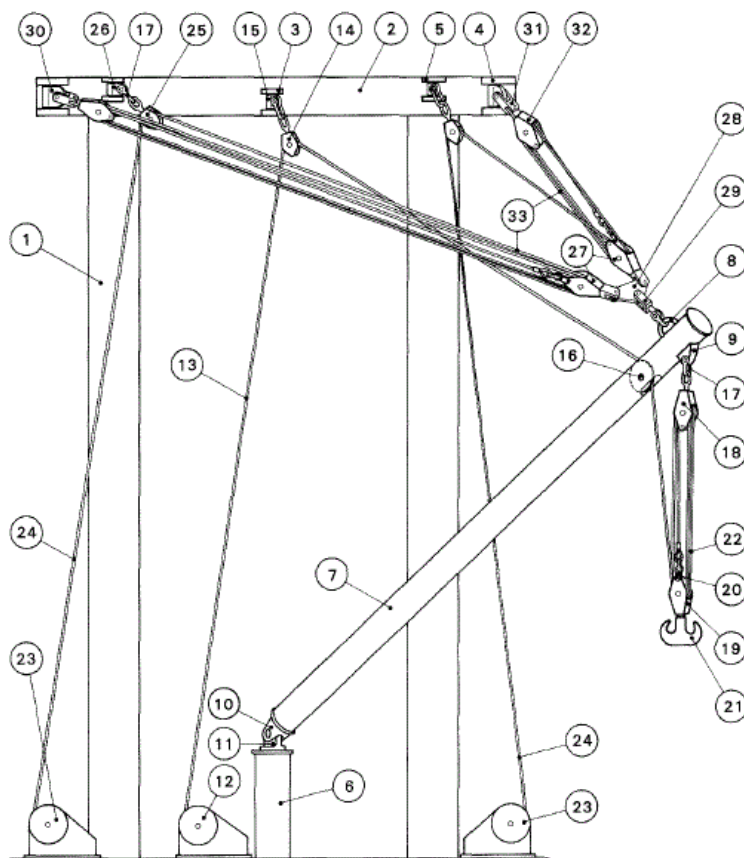
Parts Table : Twin span tackle derrick for heavy loads
