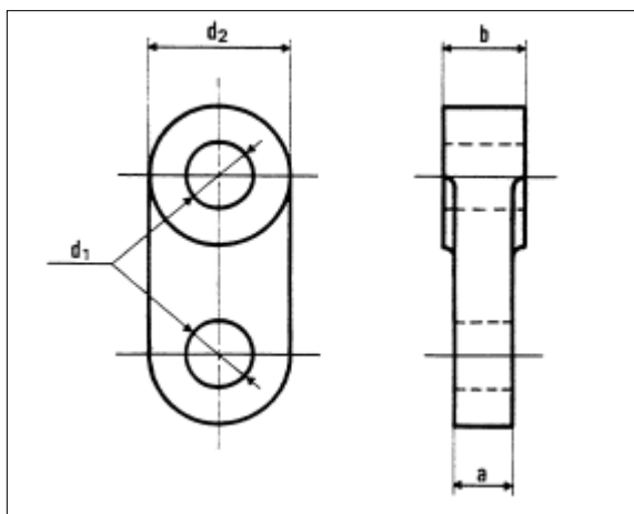
Figure 2.3.10: Becket
