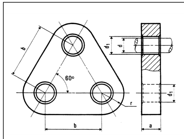
Figure 2.3.13: Triangle plate
