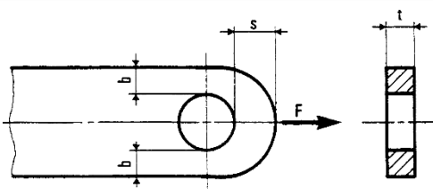
Figure 3.4.5: Hinge
