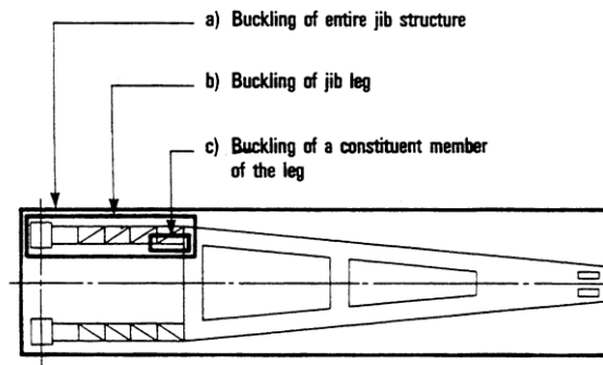
Figure 3.4.1: Verification with respect to buckling
