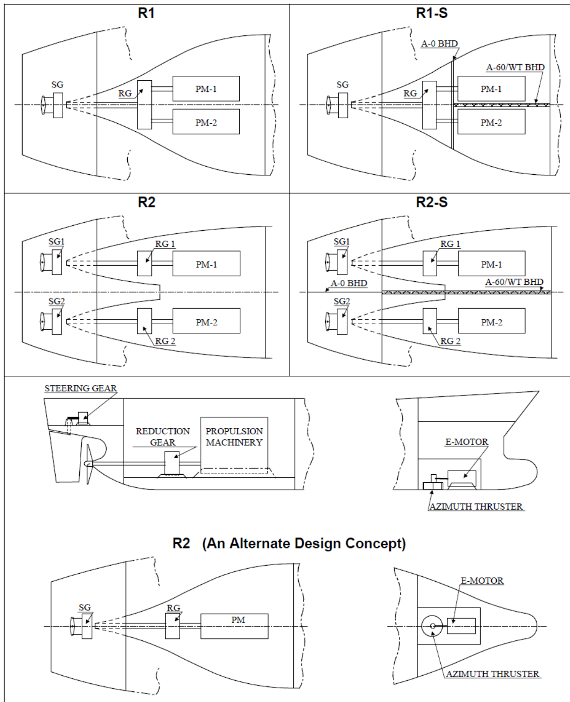
Figure 3.5.1 Arrangements of Propulsion Redundancy
