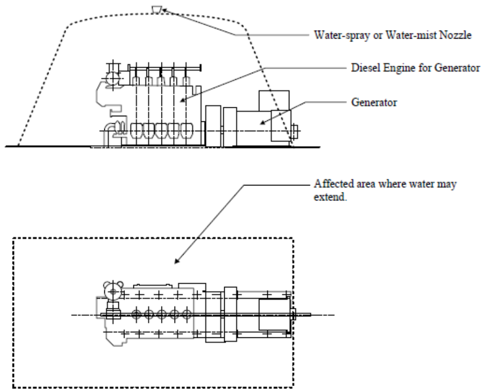
FIGURE 6.3.1 Example of Area Affected by Local Fixed Pressure Water-spraying or Local Water-mist Fire Extinguishing System in Machinery Spaces (2014)
