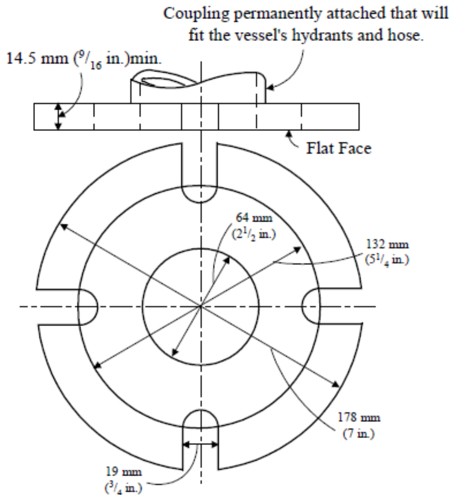
Fig 5.2.1 —international standard shore connection
