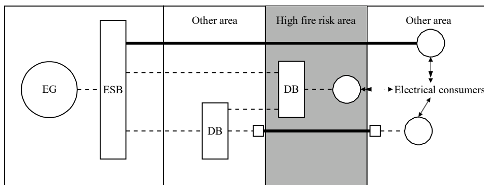
FIGURE 6.3.2 Cables within High Fire Risk Areas
