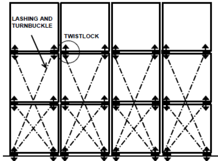
Fig 1 Individual Container Stacks with Lashings
