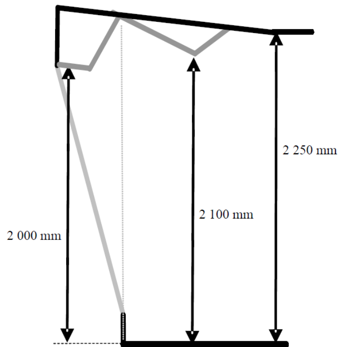
Figure 23.2.5 : Deck head height
