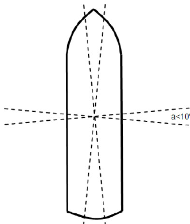
Figure 22.6.1 Sectors of ambiguity
