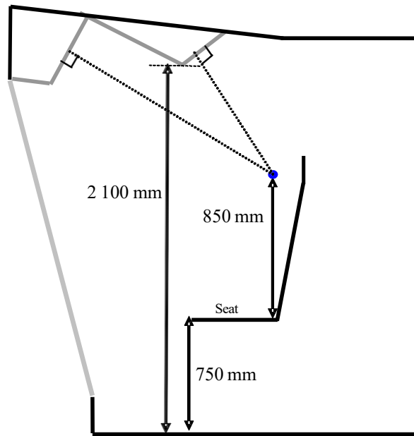
Figure 23.3.2 Overhead consoles aft
