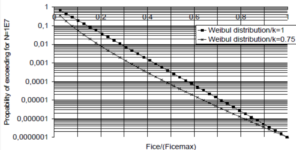
Fig. 6 The Weibull Distribution (Probability of Exceedance) for Fatigue Design
