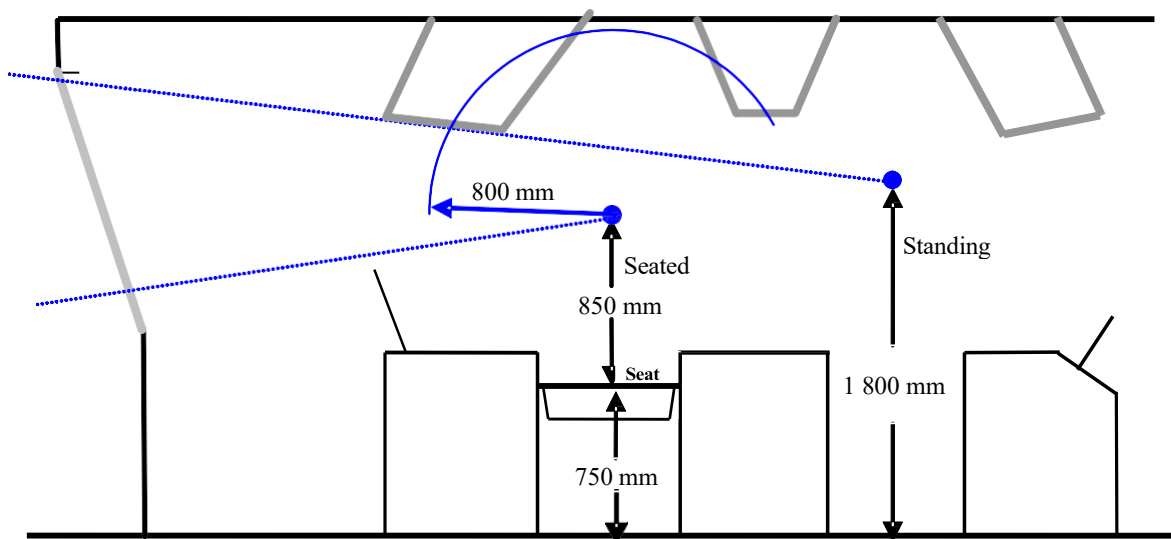
Figure 23.3.1 Overhead consoles abeam
