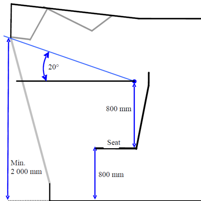
Figure 23.3.22 : Vertical field of vision in the sector of 120° astern
