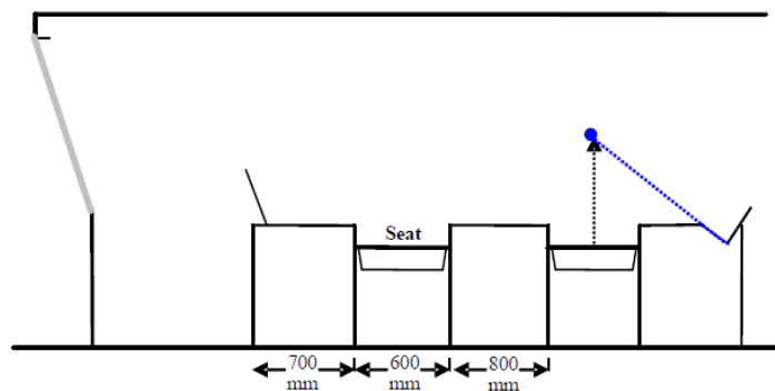
Figure 23.3.17: Size of consoles when common centre console is used
