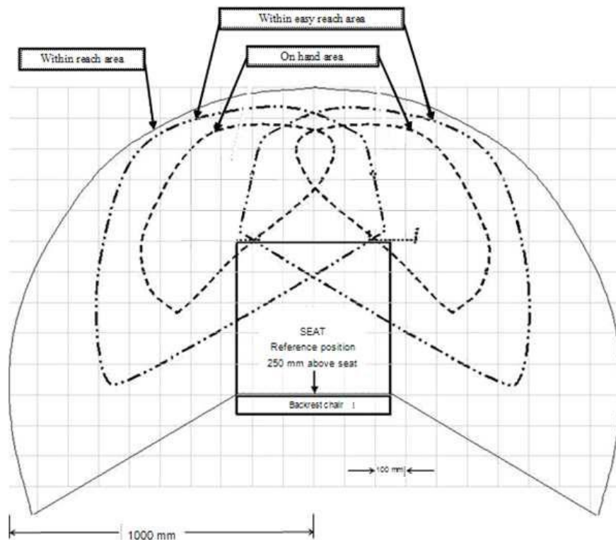
Figure 22.2.15 Areas within reach from seated position
