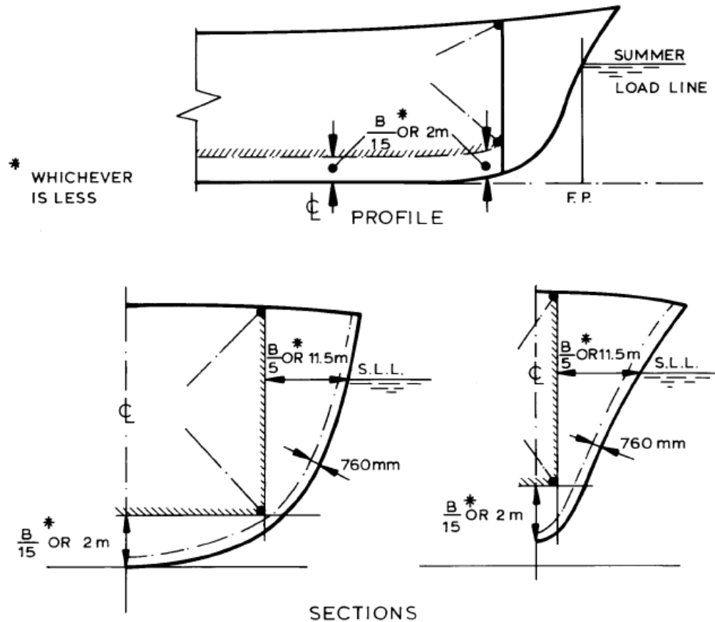
Figure 3.3.1: Tank location requirements as set out in 300
