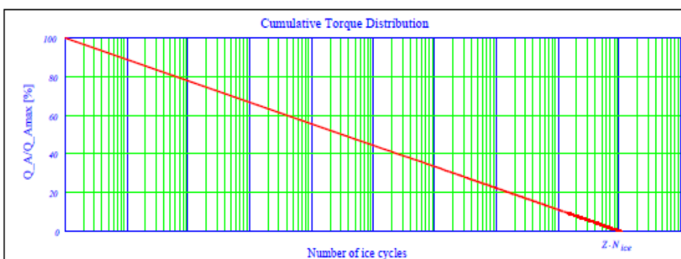
Fig. 11 Ice Load Distribution for Ducted and Open Propeller
