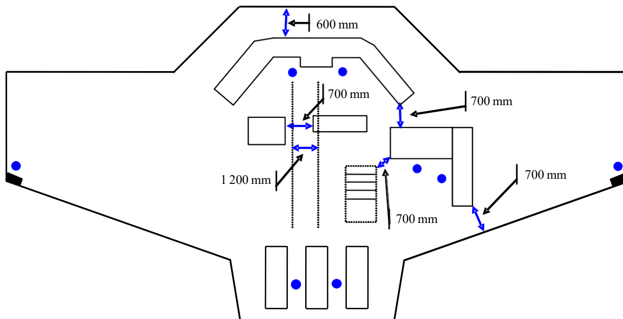
Figure 23.2.6 : Passageways between workstations
