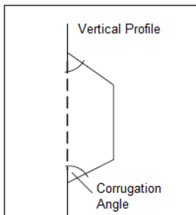
Fig 1 Definition of Corrugation Angle (Horizontally Corrugated Bulkhead)
