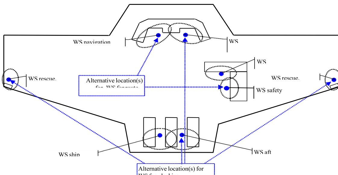
Figure 23.2.1 : Example of bridge configuration and arrangement of workstations
