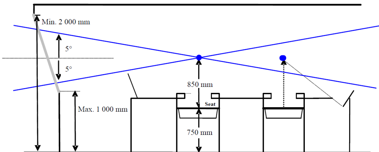
Figure 23.3.18 : Location of workstation consoles and window size in the FOV arc between abeam and 30^\circ aft of abeam.
