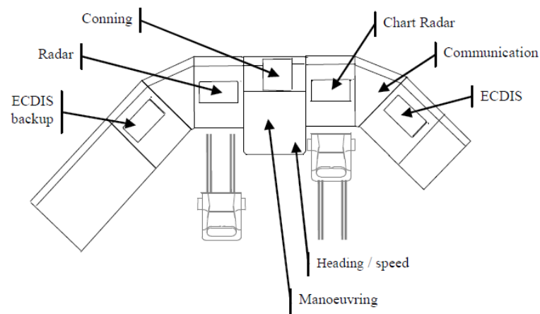
Figure 23.3.3 : Principle location of main equipment in relation to seated and standing working positions
