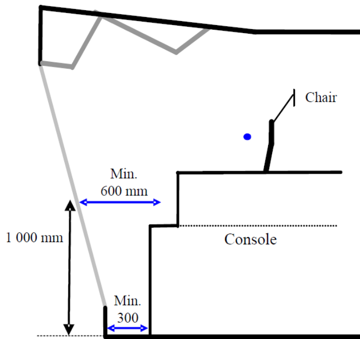
Figure 23.2.7 : Passageway between console and aft windows
