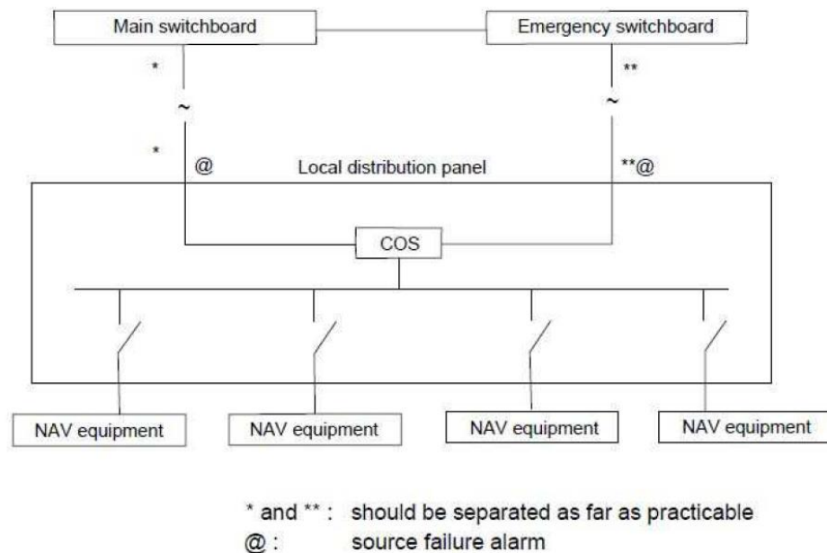
Figure 23.4. 1 Power supply for navigation equipment operated by AC
