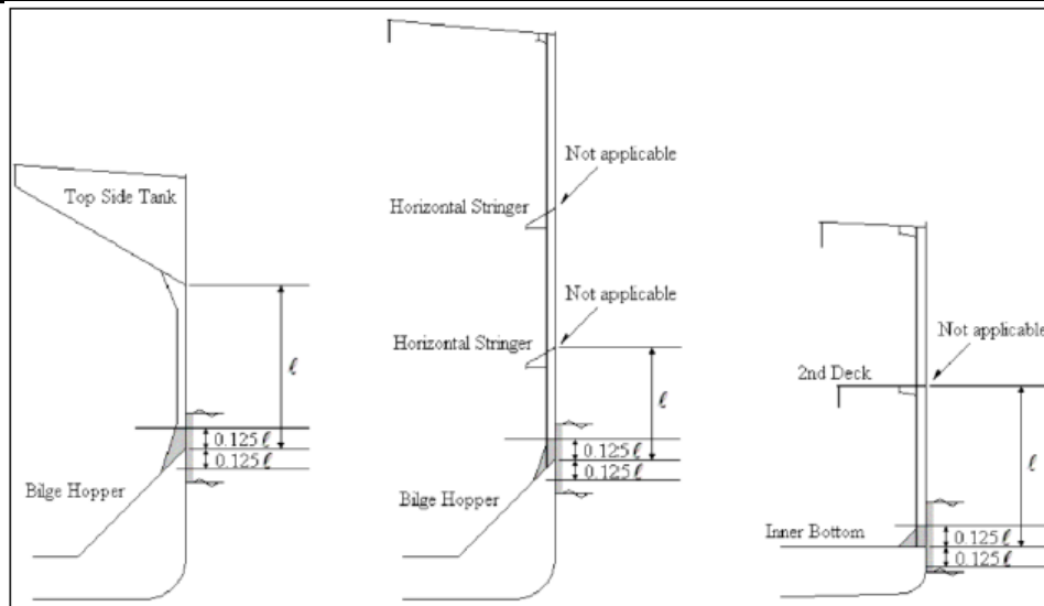
Fig 21 Side Frame Details
