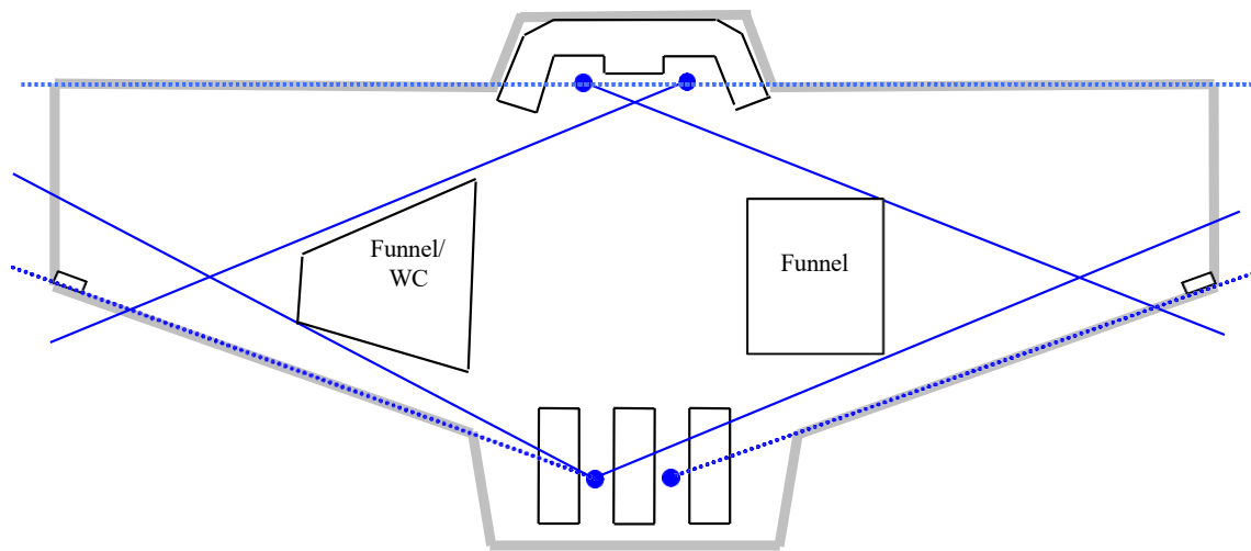
Figure 23.2.2 : Example of a bridge configuration and possible location of workstations
