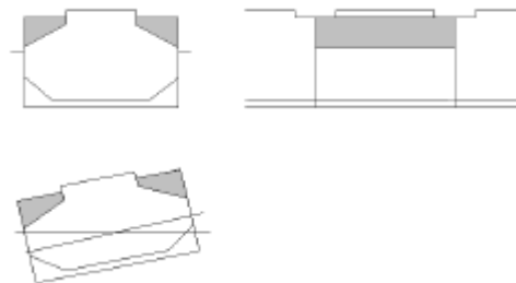
Fig 6 Ballast in Top Wing Tank
