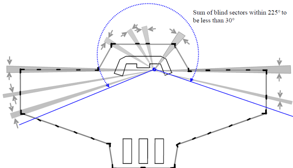
Figure 23.3.11 : Blind sectors seen from workstations for navigating & manoeuvring
