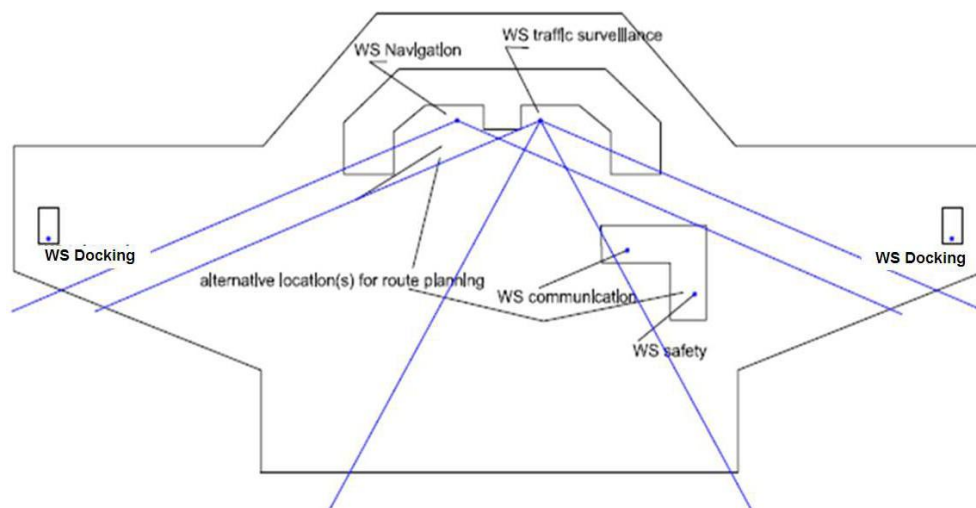
Figure 23.2.2 : Example of a bridge configuration and possible location of workstations
