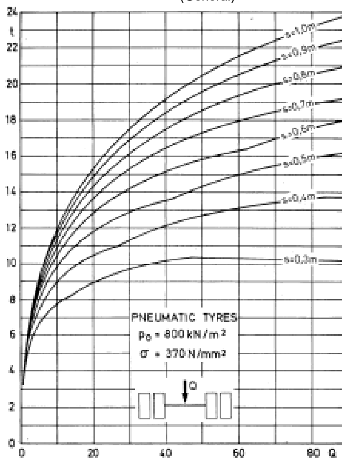
(b) Double Wheels (Axle Parallel to Stiffeners)
