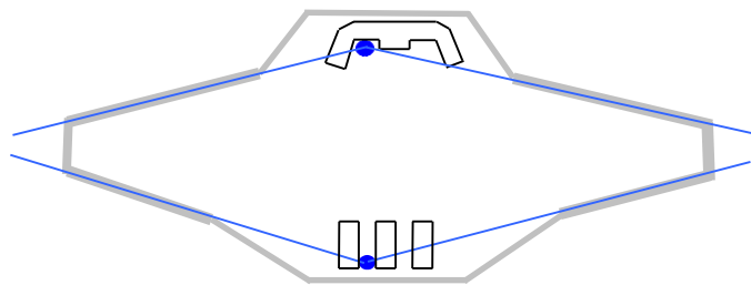
Figure 23.2.4 : Bridge bulkheads aligned with line of sight from workplaces to minimise blind sectors
