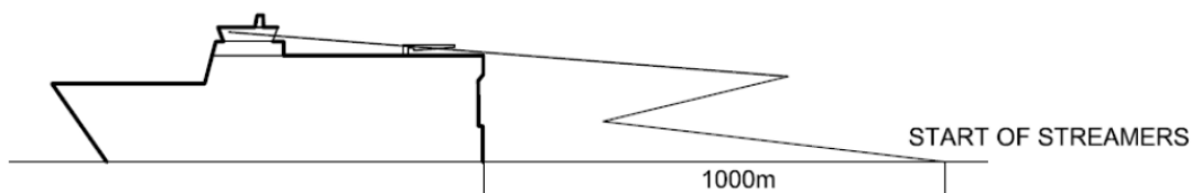
Figure 23.3.14 : Monitoring of tow for seismic vessels
