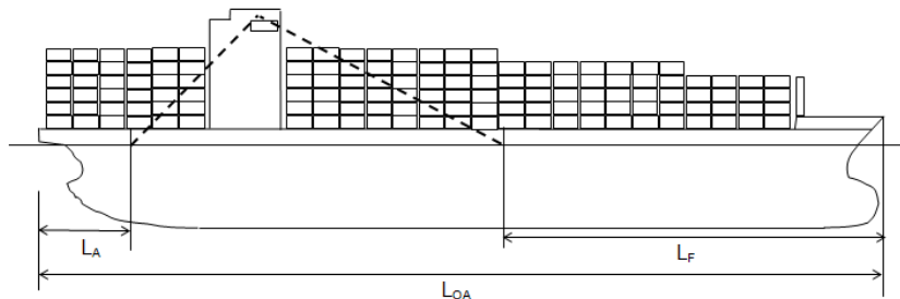
Fig. 6 Figure 22.2.6 NAUTIC-AW: View from docking station (L_A + L_F) \geq \frac{1}{2} L_{OA}
