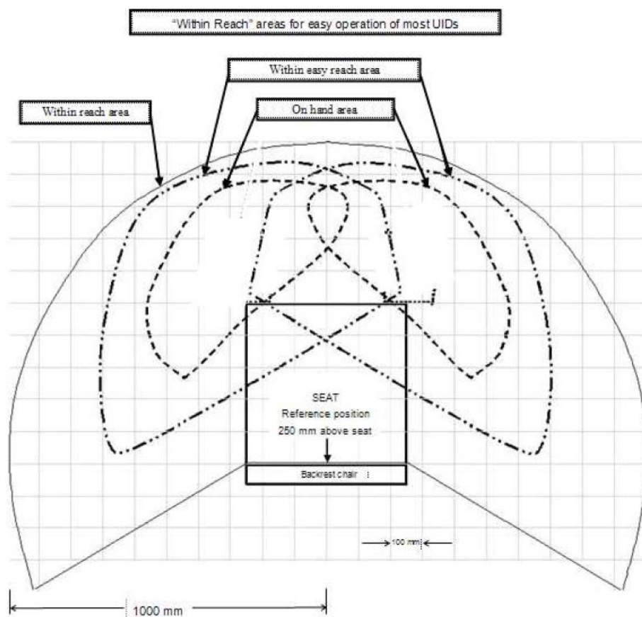
Figure 23.3.19 : Classification of reaching areas in the horizontal plane
