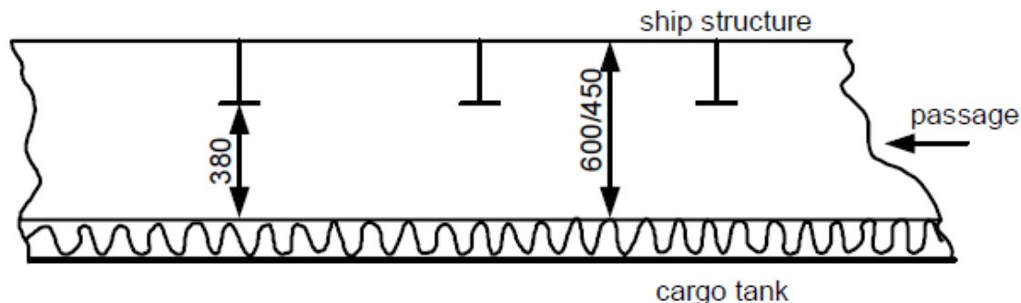
Figure 3.4.1: Minimum passage requirements involving structural elements
