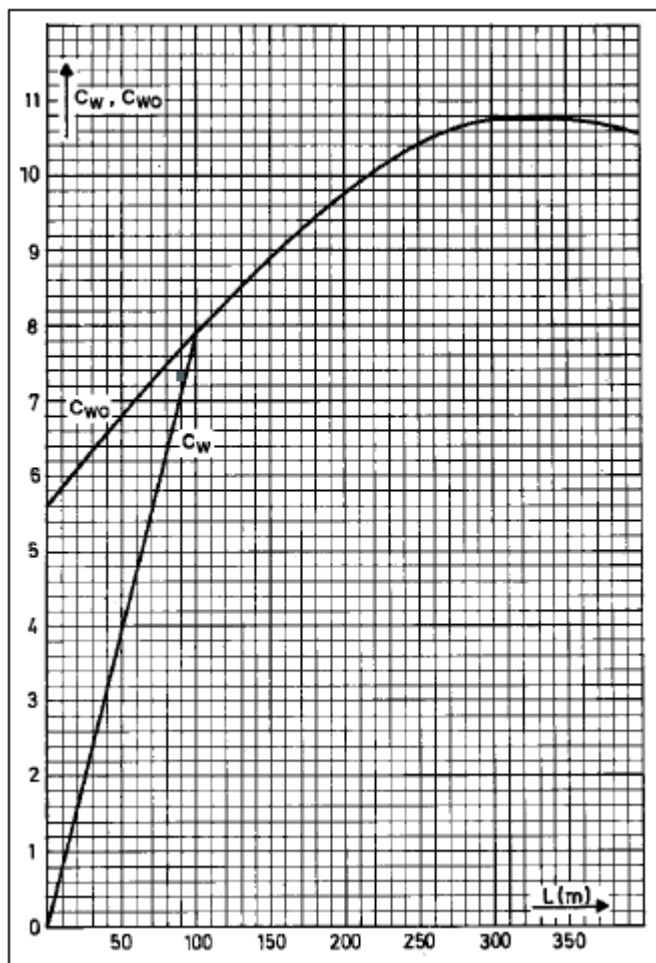
Fig 1 Wave Coefficients
