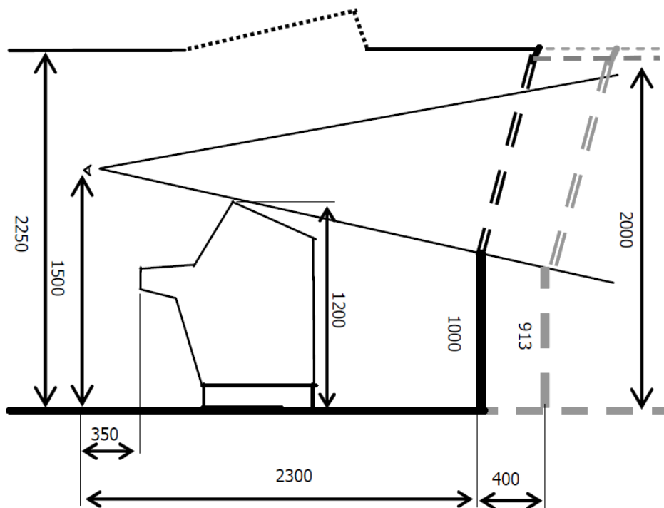
Figure 23.3.10 Vertical field of vision over consoles
