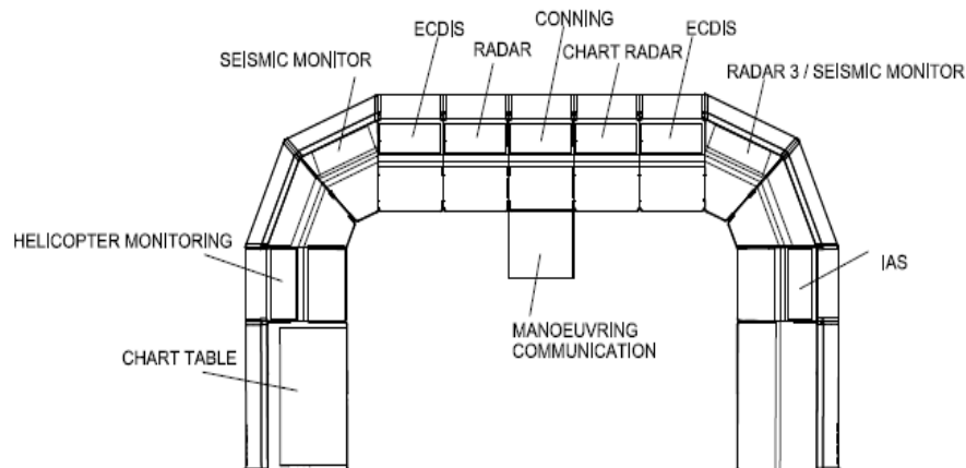
Figure 23.3.7 : Principle location of main equipment for a vessel engaged in seismic operations, overhead consoles shall also be used
