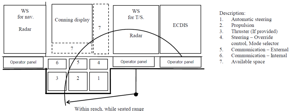
Figure 23.3.16 Example of location of important equipment
