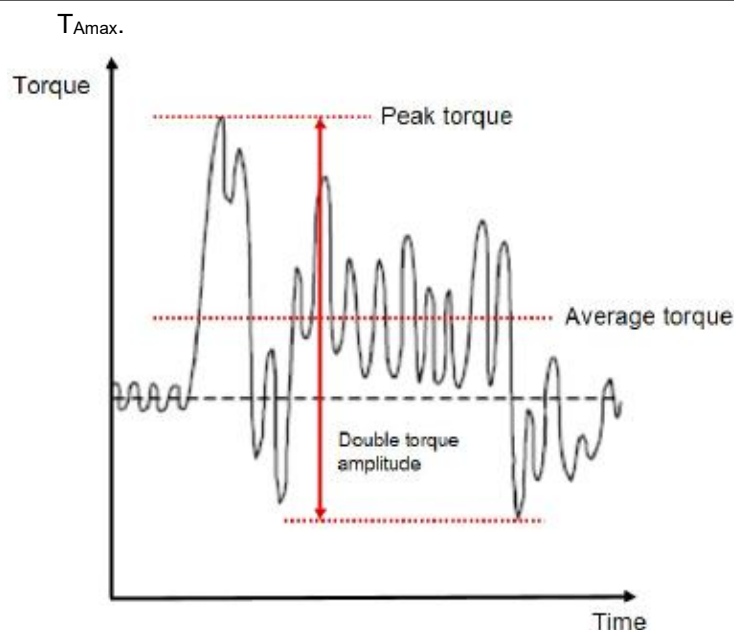
Fig. 10 Response Torque Over Time
