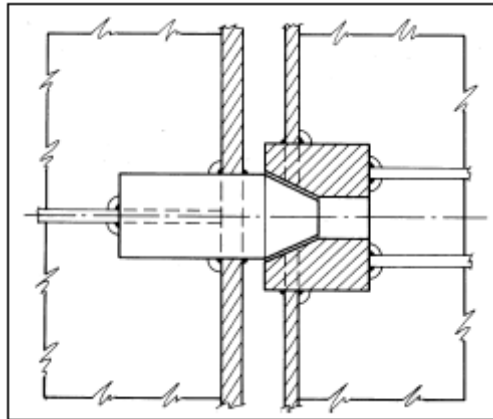
Fig 2 Thrust Bearing (Bow Door Leaves)
