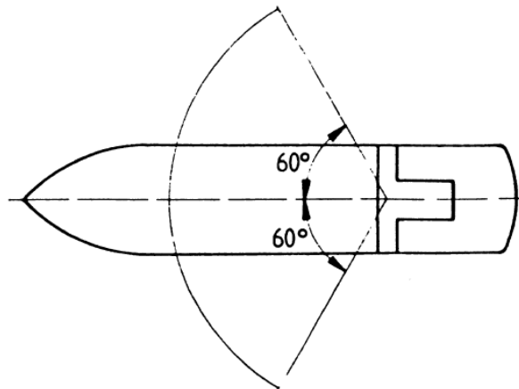
Figure 22.2.7 The field of vision from workstation for manual steering
