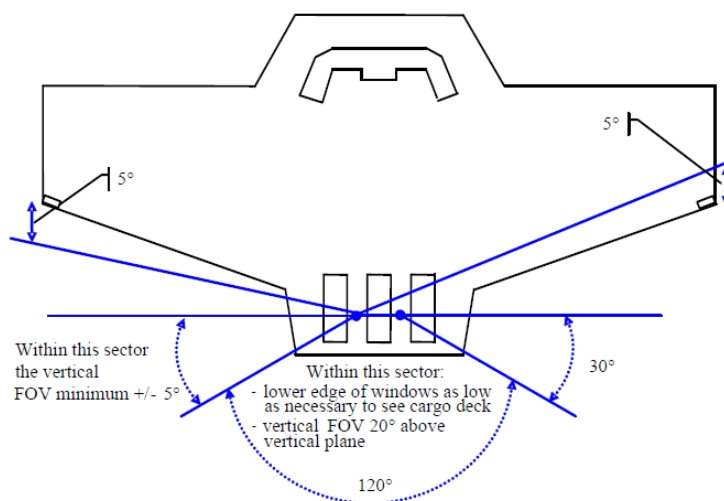
Figure 23.3.23 : Overview of the fields of vision required from workstations for offshore operations
