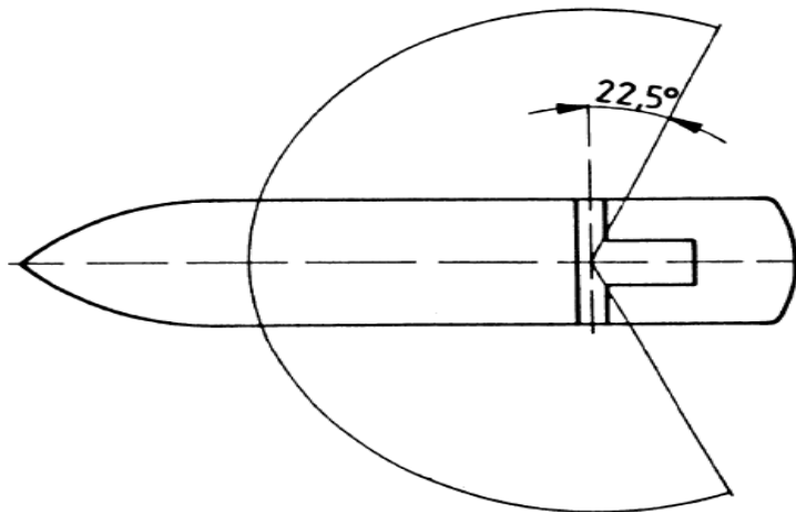
Figure 22.2.3 Horizontal field of vision from the workstations for monitoring and navigating & manoeuvring
