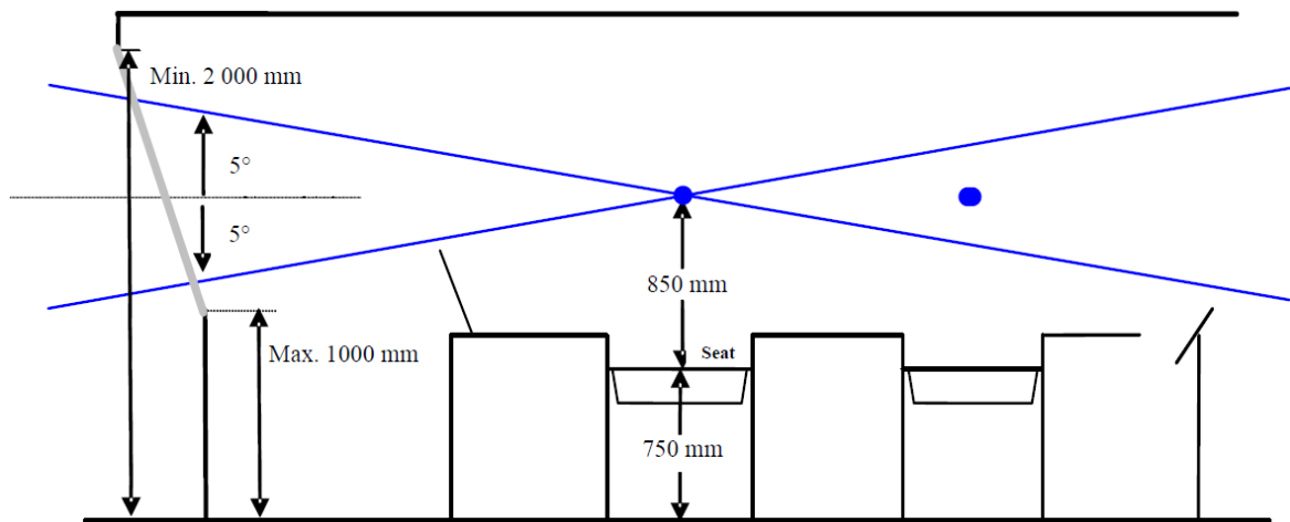
Figure 23.3.21 Vertical field of vision in the sector from abeam to 30° aft
