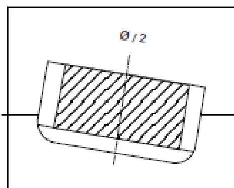
Fig 7 Heeled Loading Condition
