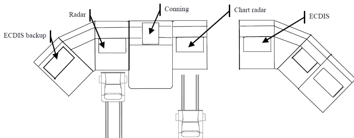
Figure 23.3.6 : Access to front windows from workstations for navigating & manoeuvring, between chart radar and ECDIS
