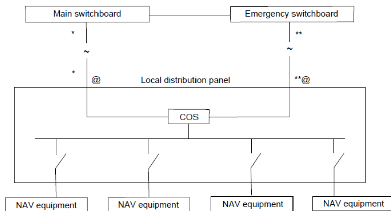
Figure 22.5.1 Power supply for navigation equipment operated by AC
