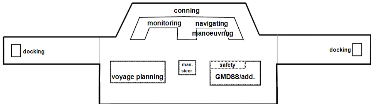
Figure .22.2.12 Design principles – typical Bridge arrangement
