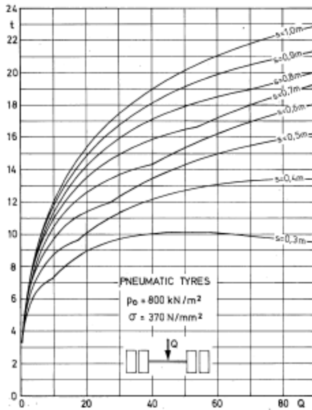
(c) Double Wheels (Axle Perpendicular to Stiffeners)
