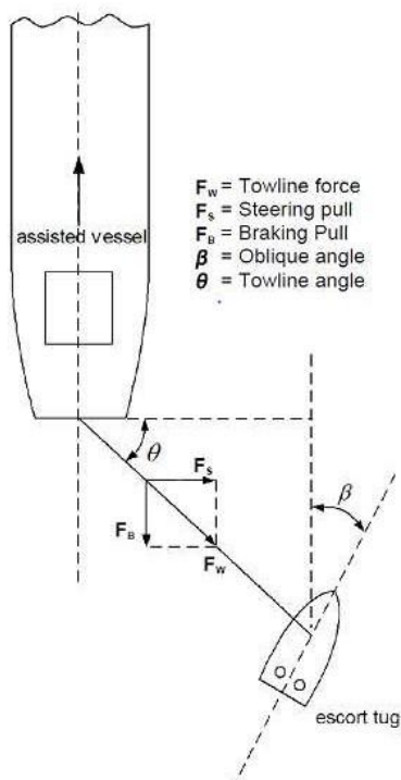
Fig. 13.1.1 Typical Escort configuration
