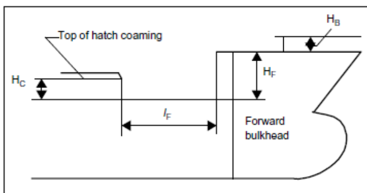
Fig 19 Forecastle Details
