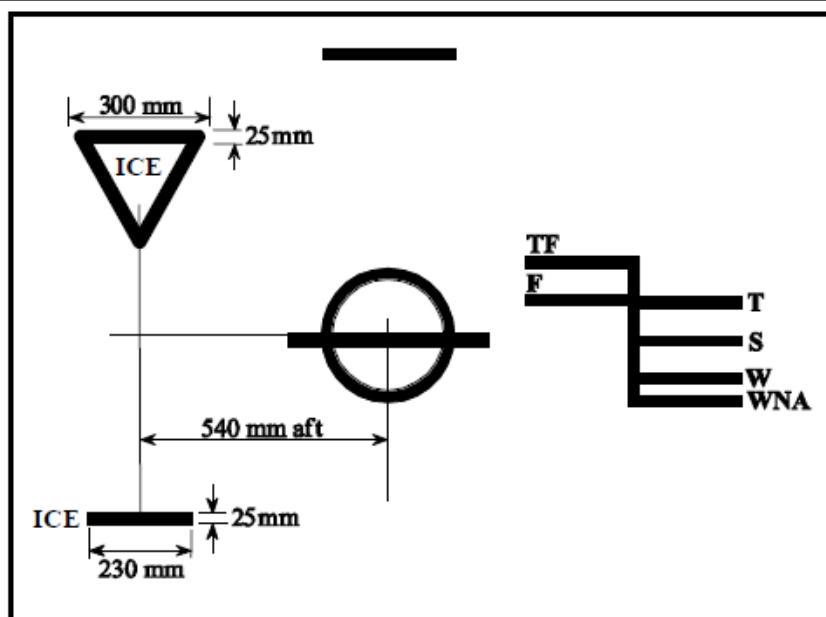
Fig. 1: Ice Class Draught Marking
