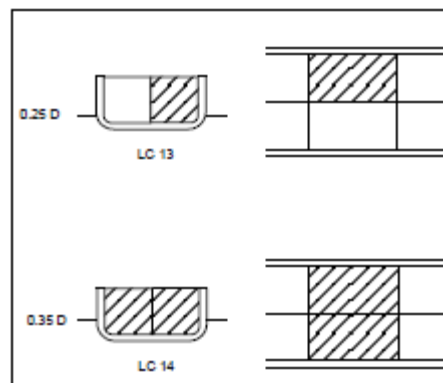
Fig 3 Seagoing Conditions for Vessels with 1 Longitudinal Bulkhead
