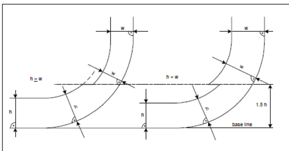
Fig 1 Double Hull Distances
