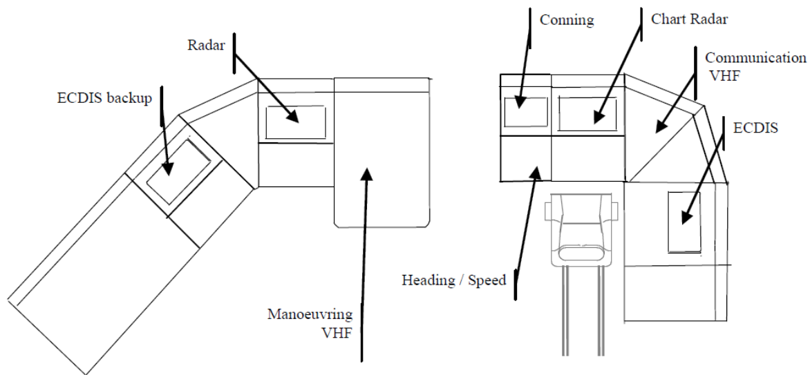
Figure 23.3.5 : Entrance to front windows may be provided from the workstations for navigating & manoeuvring
