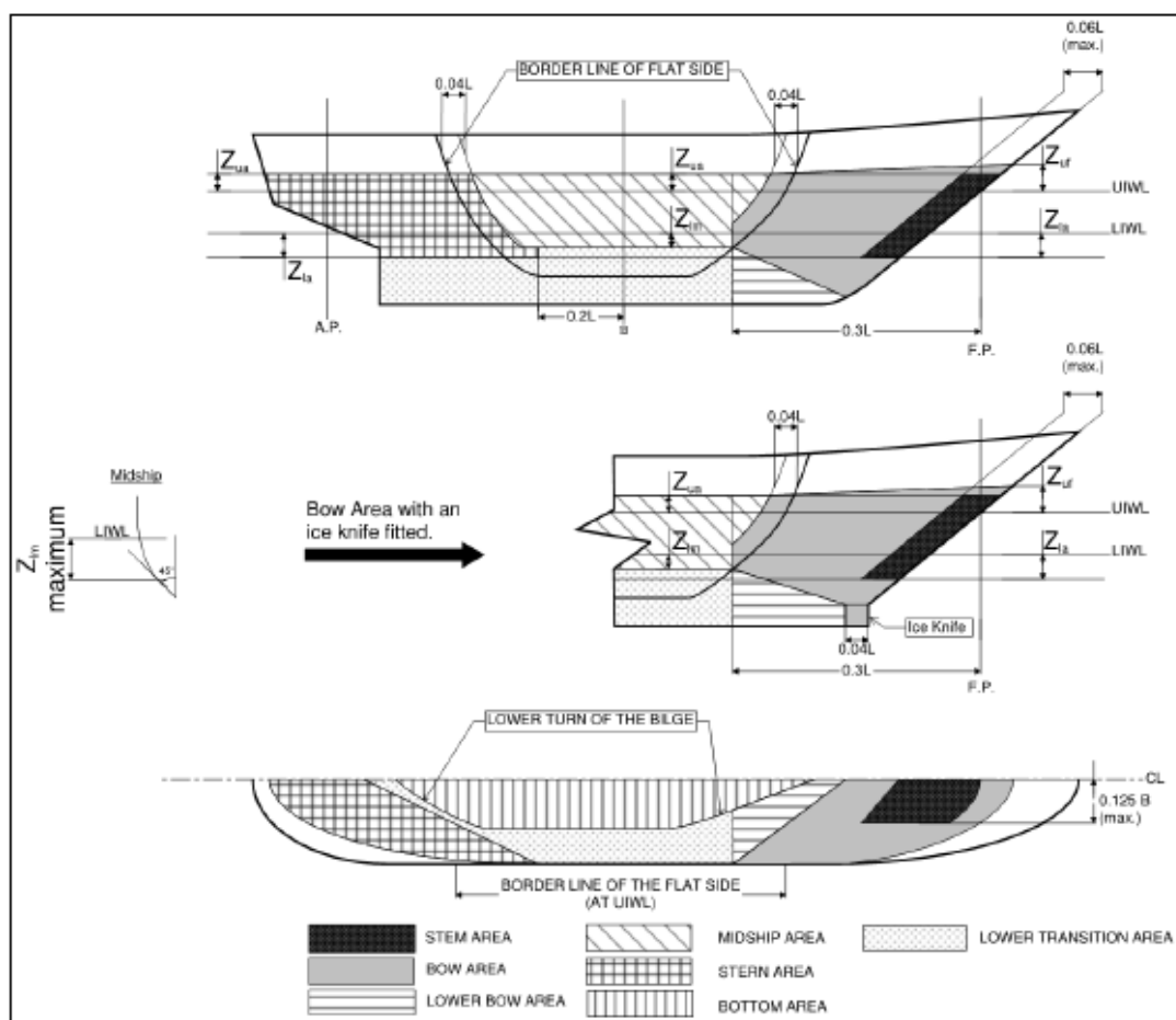
Fig.2 Ice Reinforced Area
